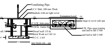
SEPTIC TANK WITH DISPENSER
