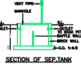
SECTION OF SEP. TANK
