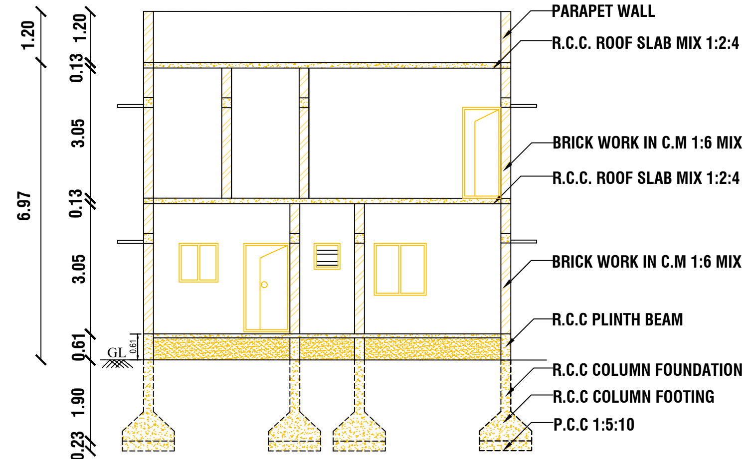
CROSS SECTION AT A-A
