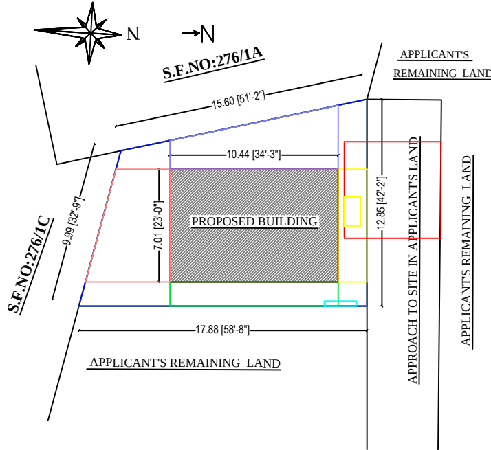
PROPOSED PLAN
