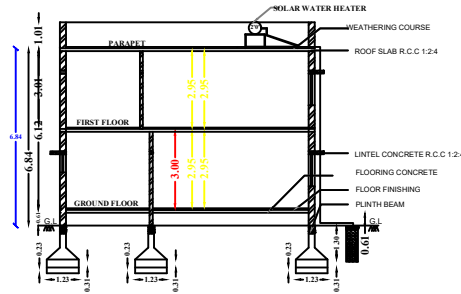
SECTION
