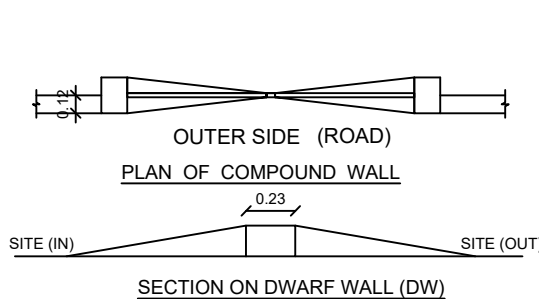
OR PLAN
