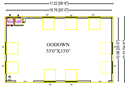
PROPOSED GODOWN BUILDING
