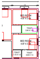
FLOOR PLAN
