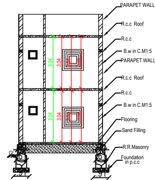
SECTION AB
