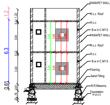
SECTION ,AB
