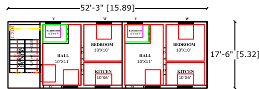
GROUND FLOOR PLAN
