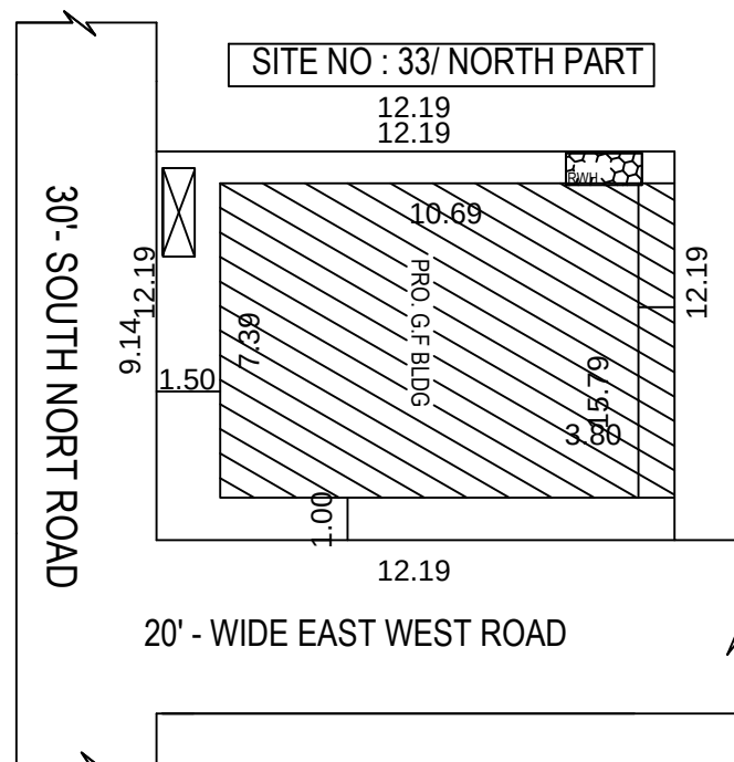
SITE PLAN
