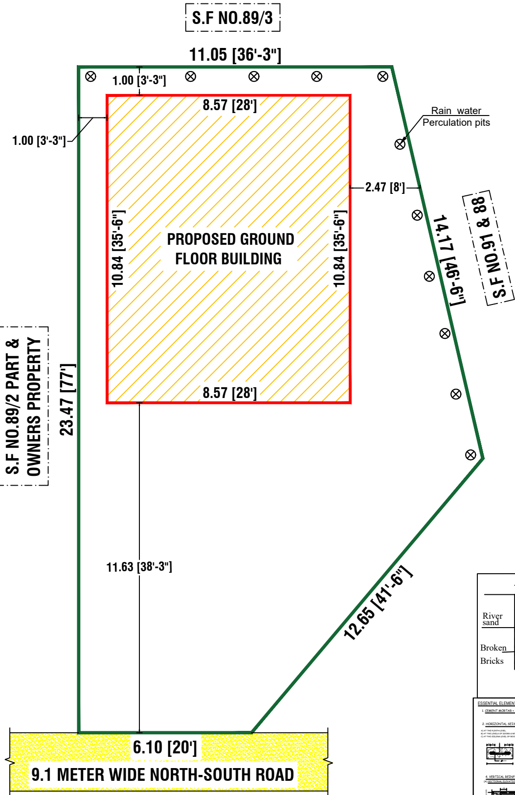
SITE PLAN
