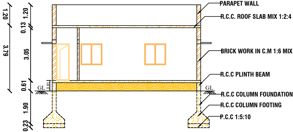
CROSS SECTION AT A-A
