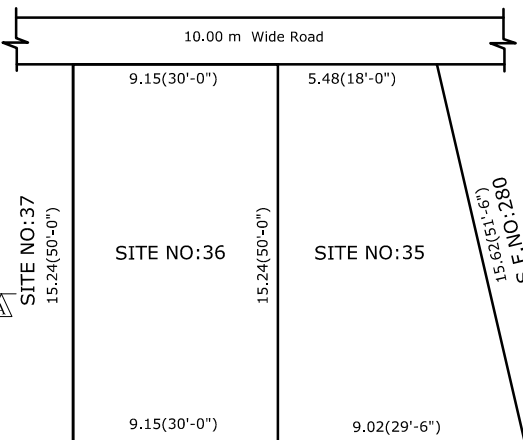
RECONSTITUTION PLAN
