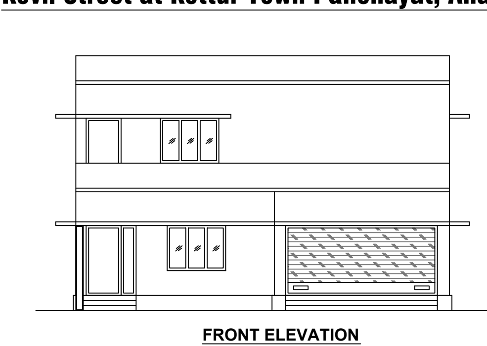
FRONT ELEVATION
