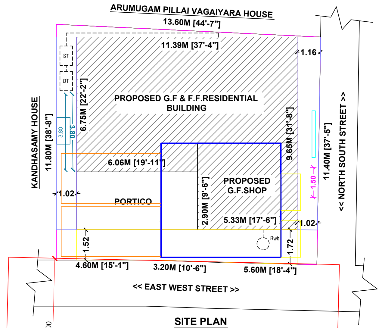
SITE PLAN
