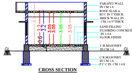
CROSS SECTION
