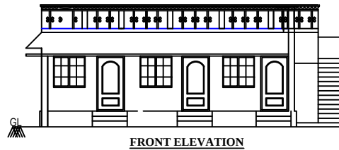
FRONT ELEVATION
