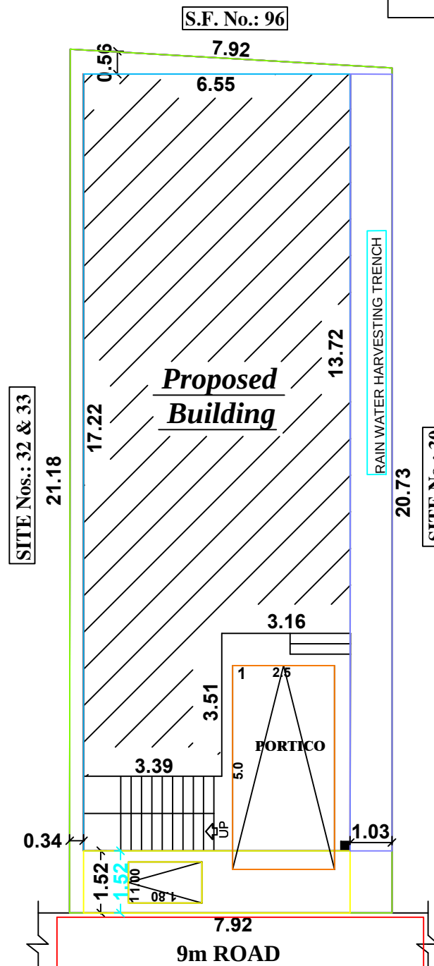
SITE PLAN
