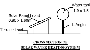
CROSS SECTION OF SOLAR WATER HEATING SYSTEM
