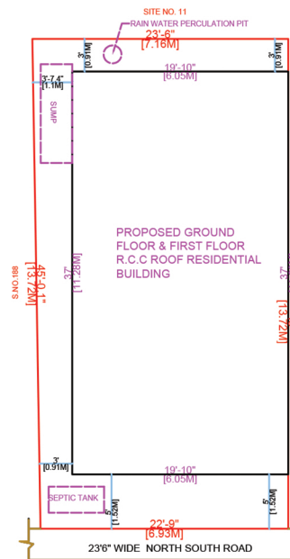
SITE PLAN
