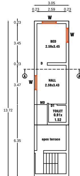
ADD. PROPOSED FIRST FLOOR
