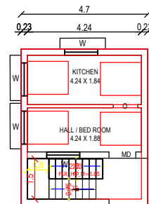
PROPOSED FIRST FLOOR BUILDING
