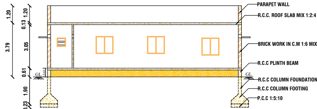
CROSS SECTION AT A-A
