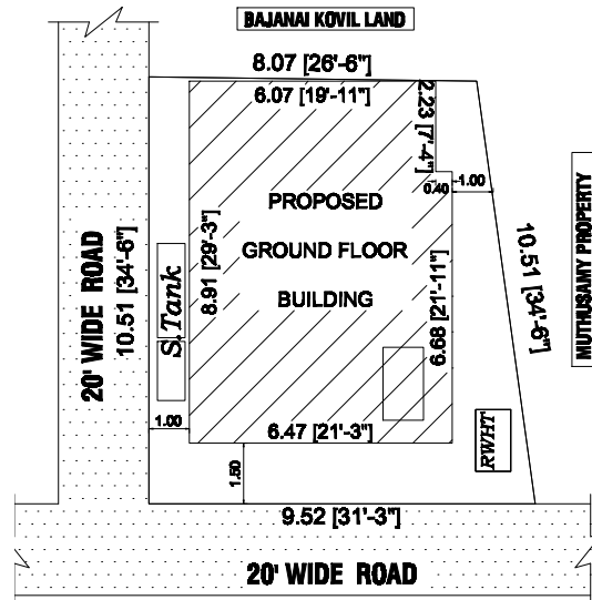
SITE PLAN
