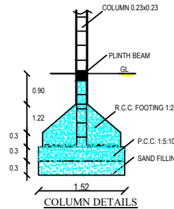
COLUMN DETAILS
