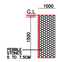
SECTION OF PEBBLE TRENCH SCALE : 1: = 100
