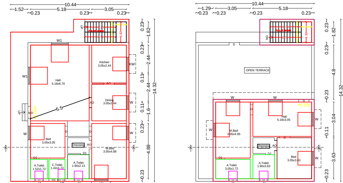
PROPOSED FIRST FLOOR SCALE 1:100
