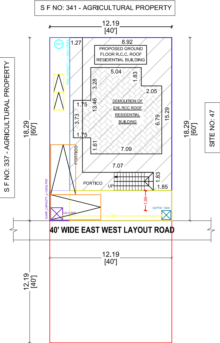
SITE PLAN
