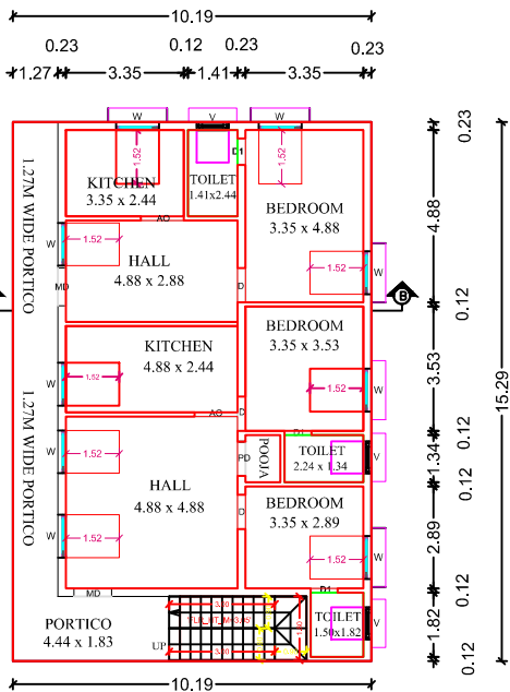
D GROUND FLOOR PLAN
