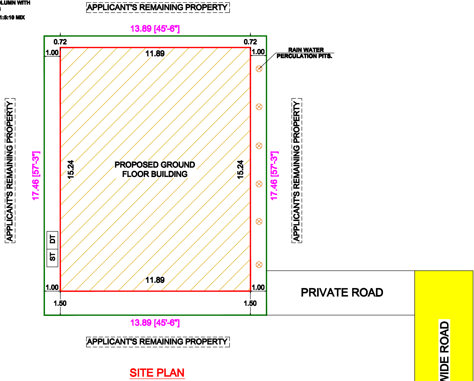
SITE PLAN
