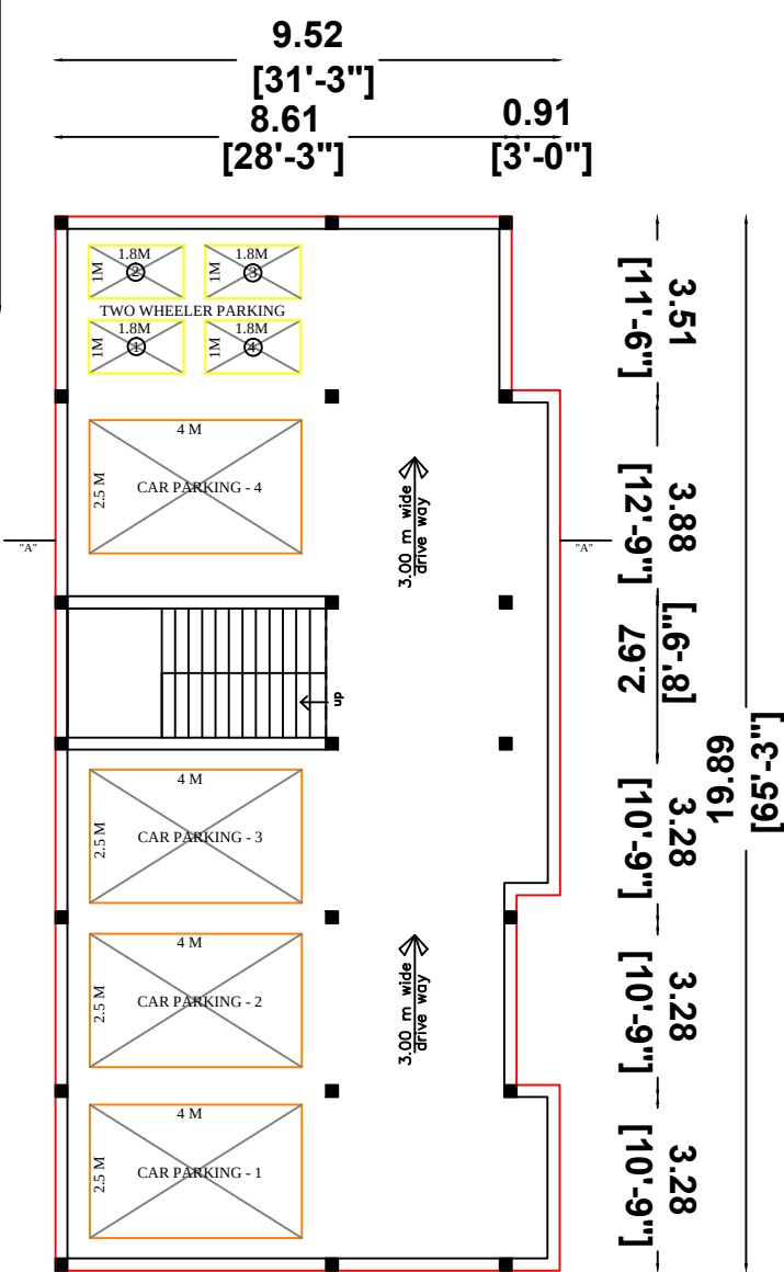
STILT/GROUND FLOOR PLAN
