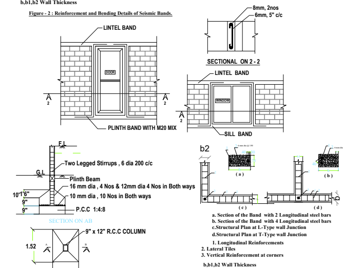
Figure - 3 : Typical Details of Providing Vertical Steel Bars in Brick Masonry.
