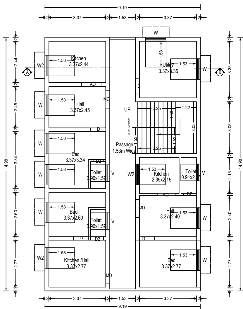
Plan Scale 1:100 Exg.First floor
