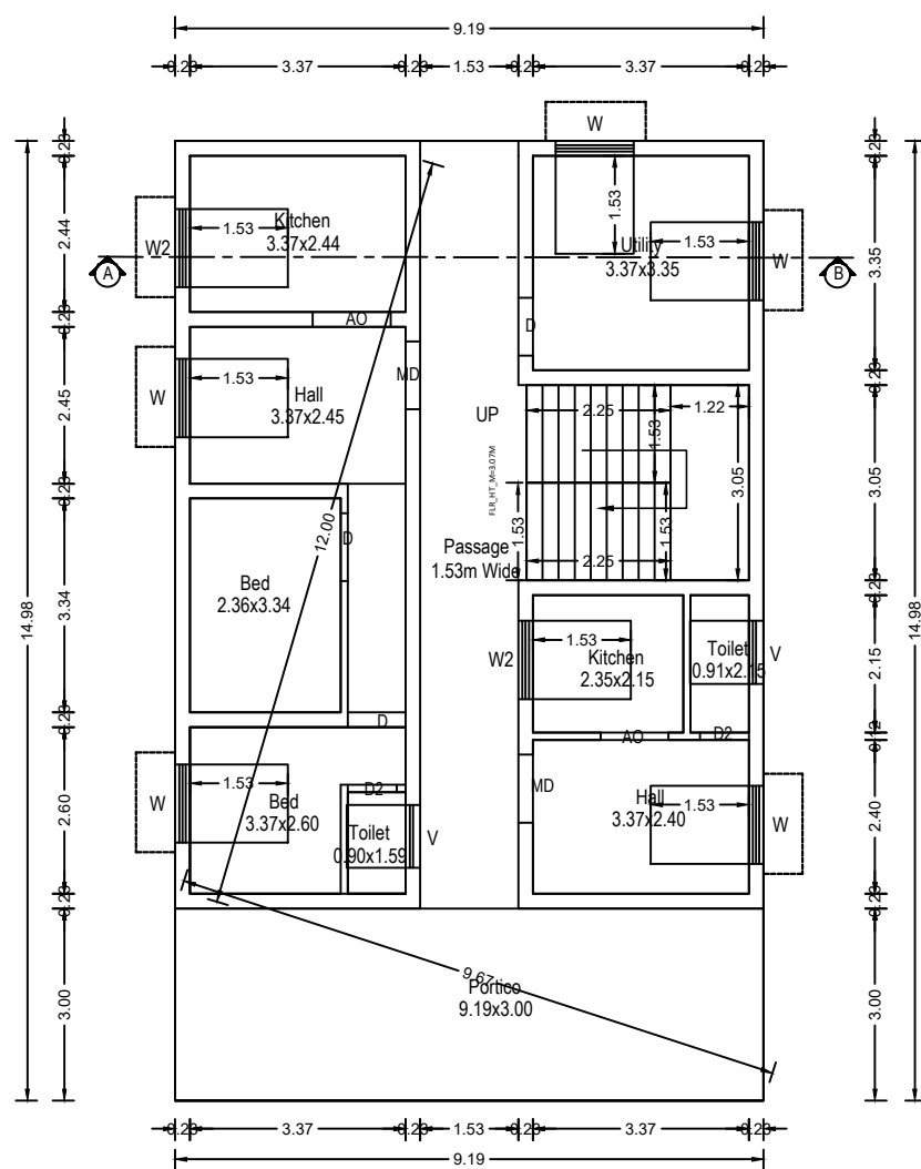
Plan Scale 1:100 Exg.Ground floor
