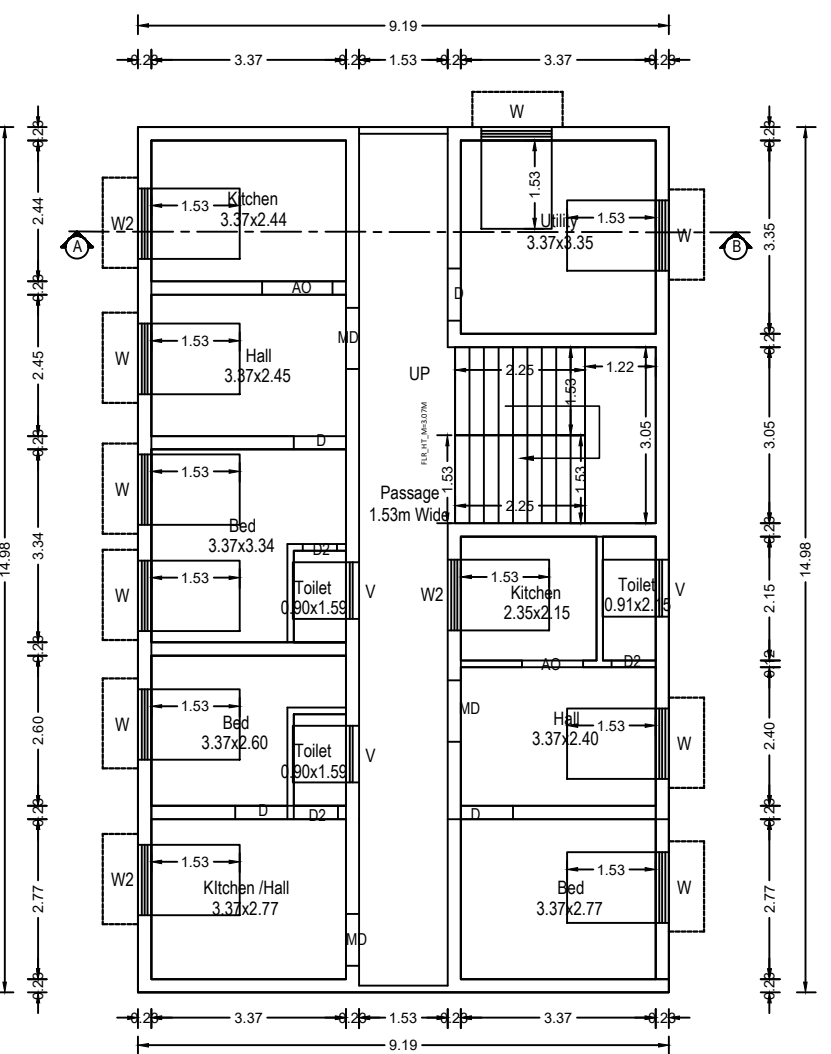
Plan Scale 1:100 Pro.Second floor
