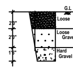
TRIAL PIT
