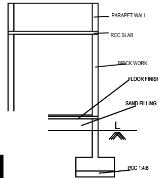
CROSS SECTION ON A-B
