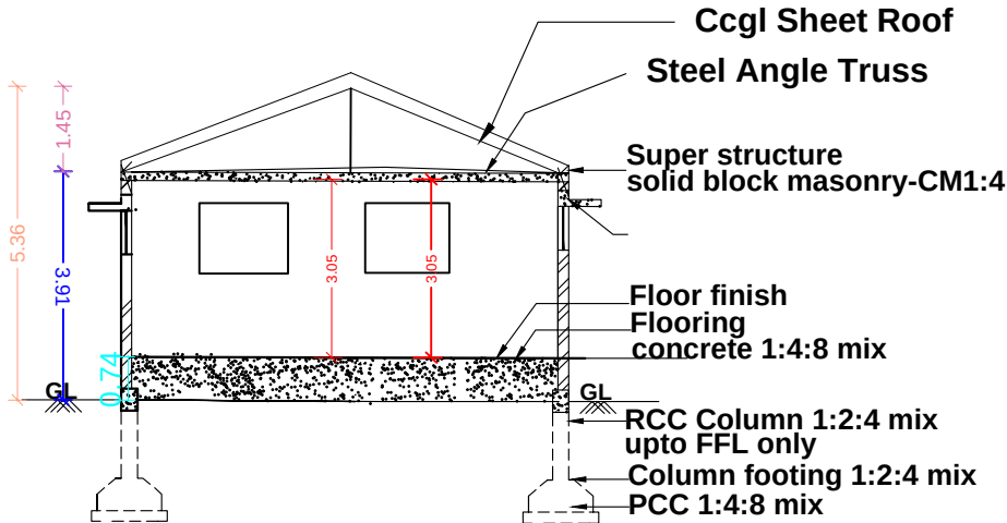
SECTION ELEVATION
