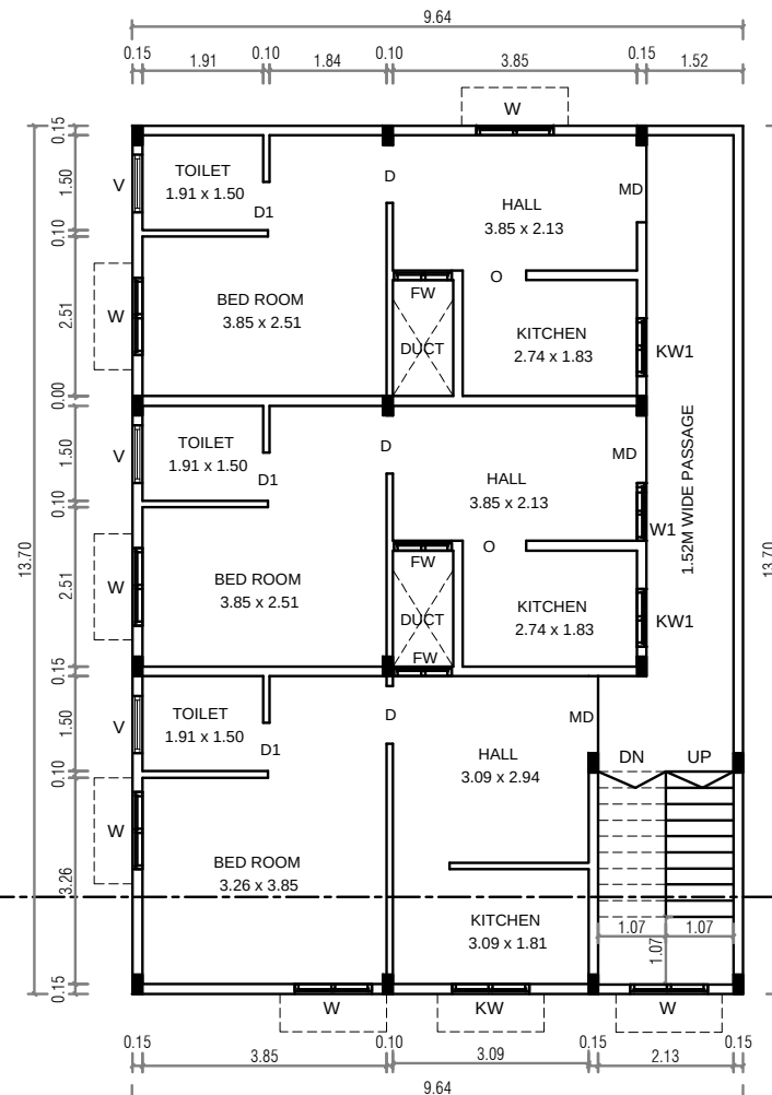
FIRST &amp; SECOND FLOOR PLAN
