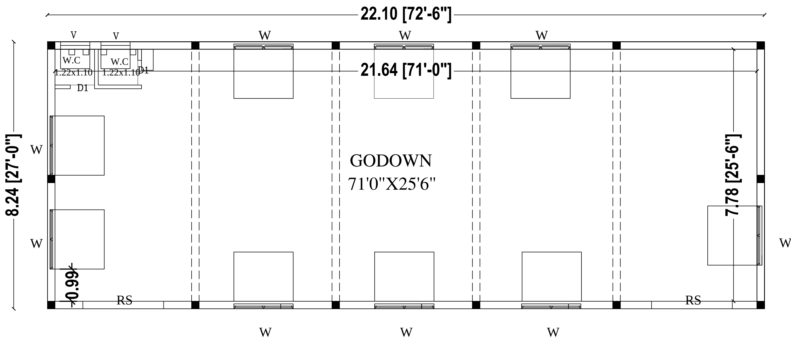
PROPOSED PLAN
