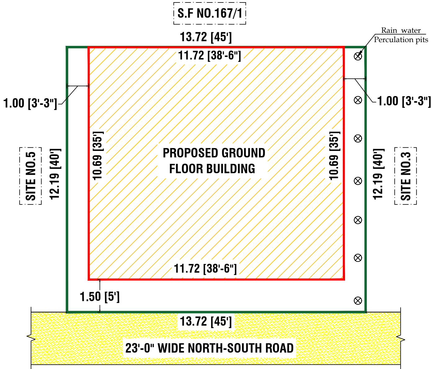
SITE PLAN
