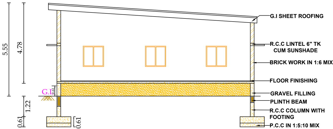
CROSS SECTION AT A-A
