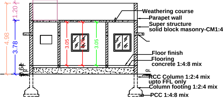
SECTION ELEVATION
