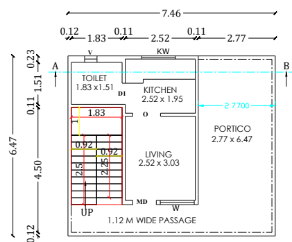
EXTG.G.FLOOR PLAN (ALTERATION)
