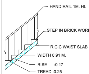
STAIR DETAIL
