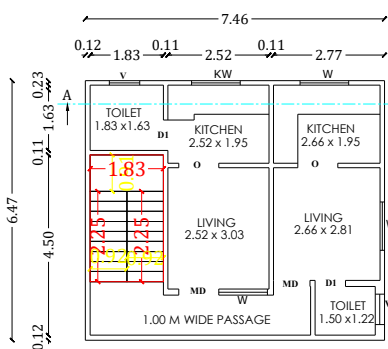
PRO.SECOND FLOOR
