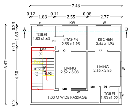
EXTG.F.FLOOR PLAN (ALTERATION)
