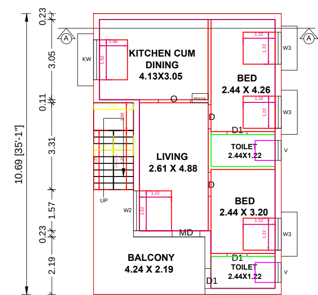
PRO. FIRST FLOOR PLAN
