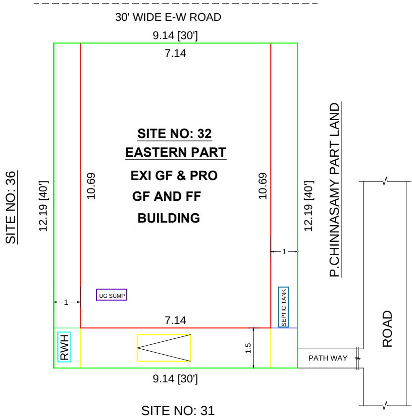
SITE PLAN
