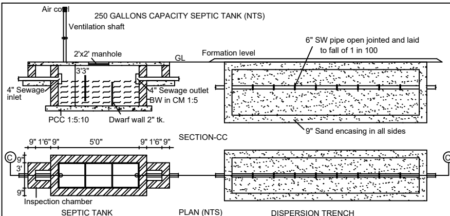
SEPTIC TANK PLAN (NTS) DISPERSION TRENCH
