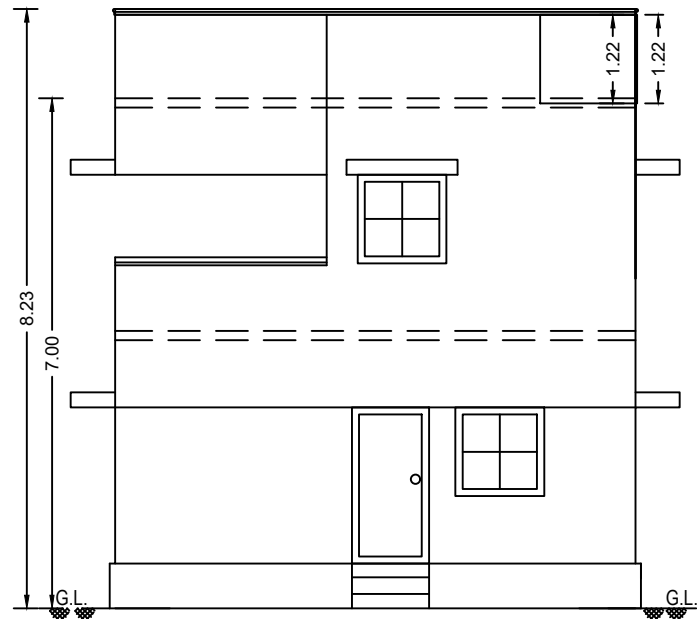
Elevation (East - Side)
