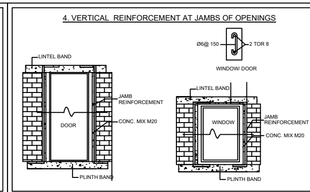
3. VERTICAL REINFORCEMENT IN BRICK WALLS 4. VERTICAL REINFORCEMENT AT JAMBS OF OPENINGS
