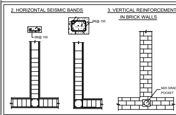
2. HORIZONTAL SEISMIC BANDS
