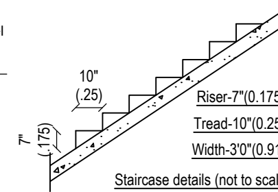
Staircase details (not to scale)
