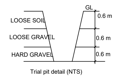
Trial pit detail (NTS)
