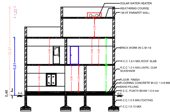
SECTION AT ( B - B )
