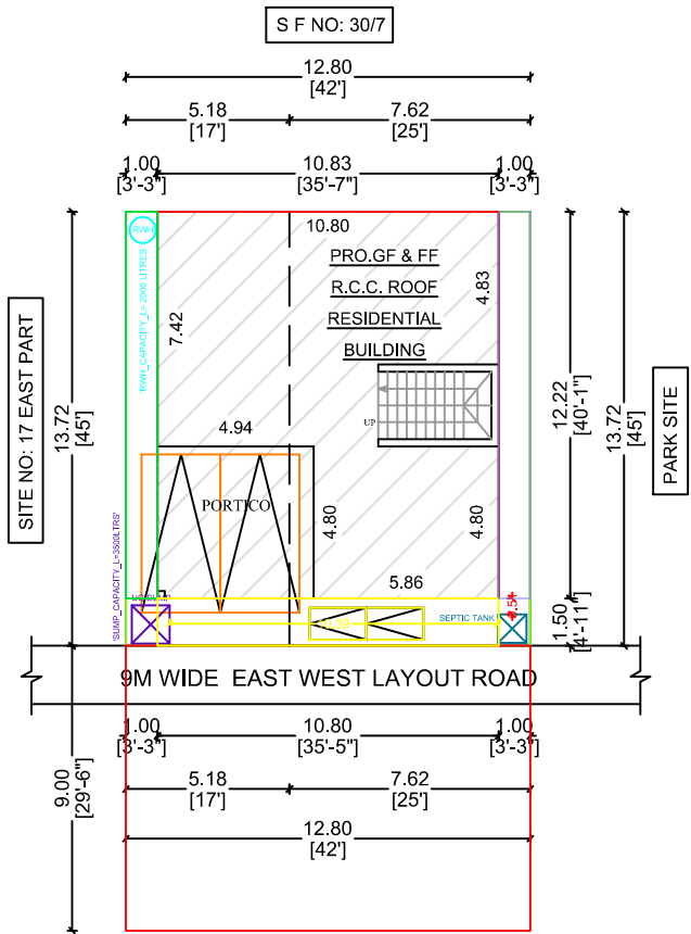
SITE PLAN
