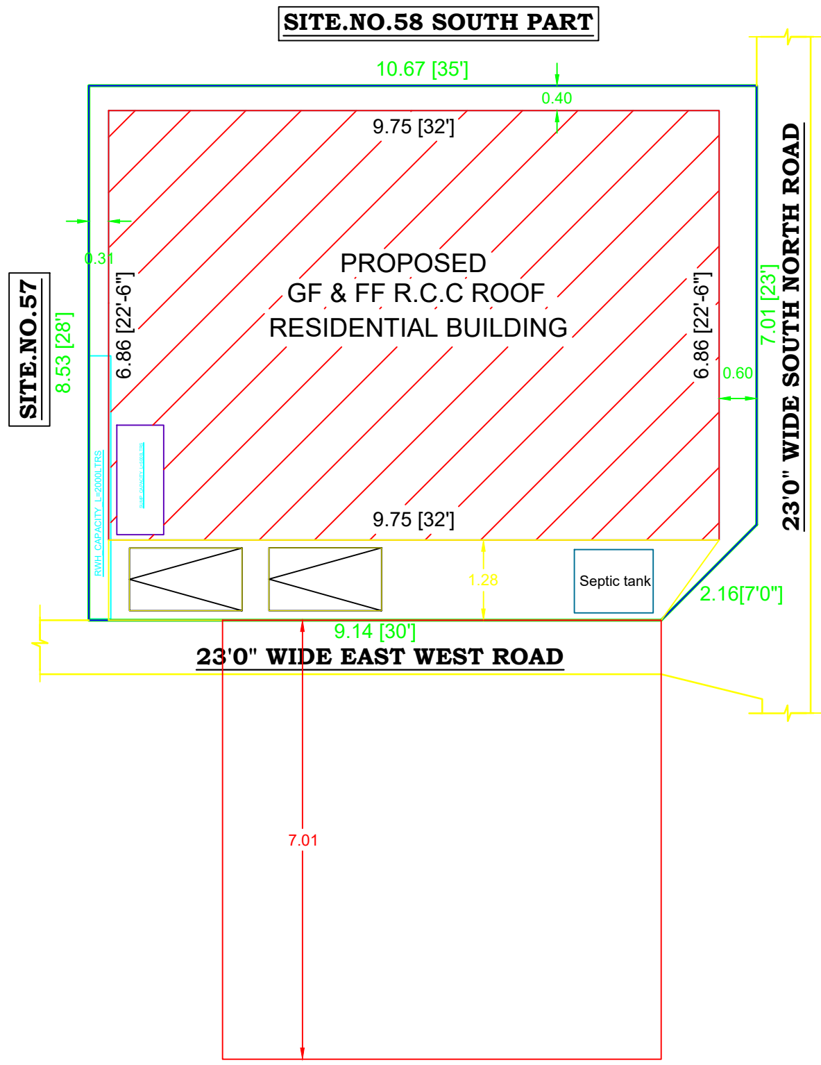
SITE PLAN
