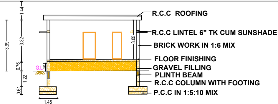
CROSS SECTION AT A-A
