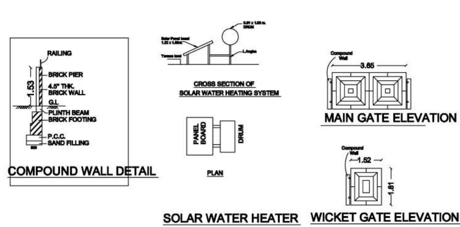
COMPOUND WALL DETAIL. SOLAR WATER HEATER. WICKET GATE ELEVATION. MAIN GATE ELEVATION.
