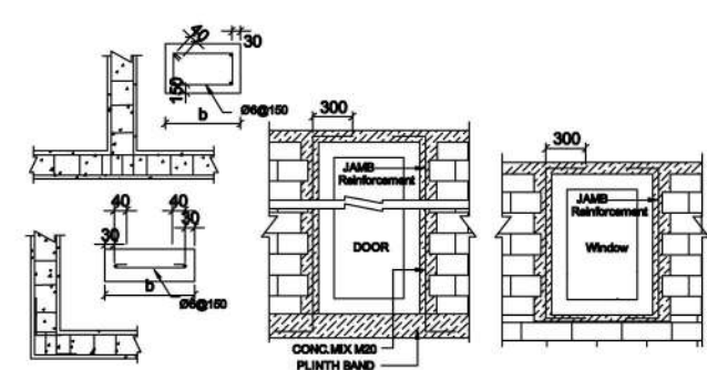
Typical Details of Providing Reinforcement & Bending Details of Seismic Bands. Vertical steel Bars around doors/windows. ESSENTIAL INTERNAL ELEMENTS IN BUILDING.
