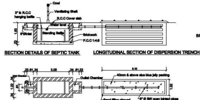
SECTION DETAILS OF SEPTIC TANK. LONGITUDINAL SECTION OF DISPERSION TRENCH. PLAN OF SEPTIC TANK. DISPERSION TRENCH (TYP). DETAILS OF SEPTIC TANK - 250 GALLONS.
