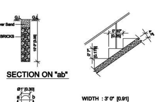
SECTION ON "ab". RAIN WATER PERCOLATION PIT. STAIRCASE DETAILS: WIDTH : 3' 0" [0.91]. RAISER : 0' 7" [0.175]. TREAD : 0' 10" [0.25].
