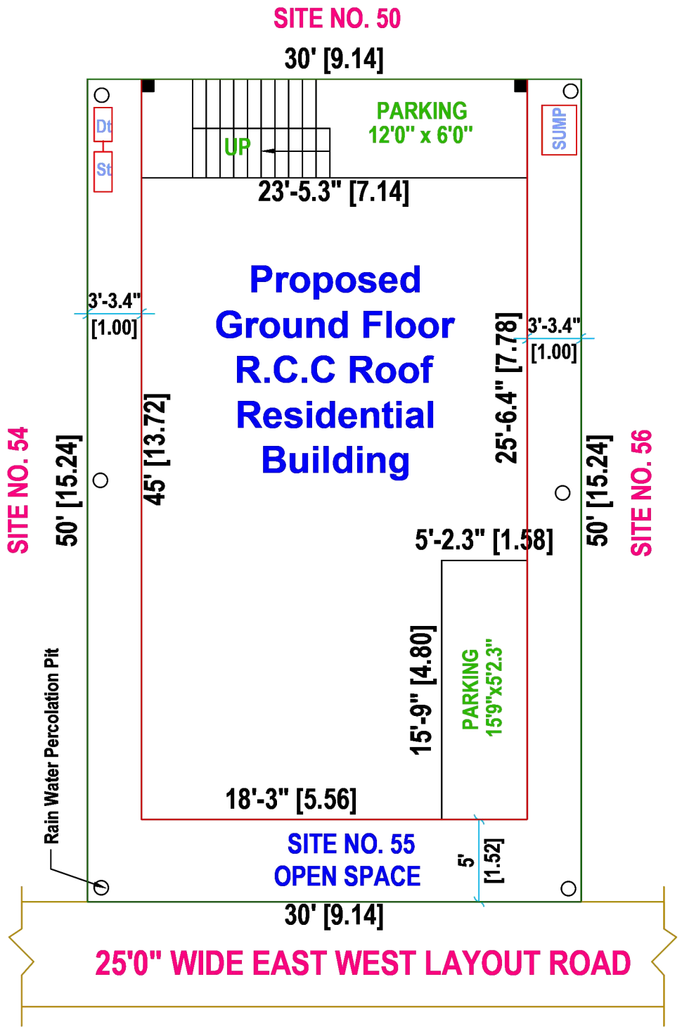
SITE PLAN (SCALE 1" : 8' 0")
