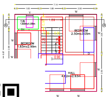
F FLOOR PLAN
