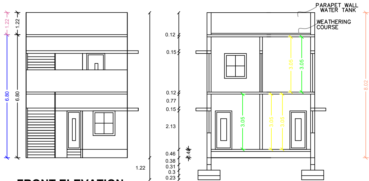
FRONT ELEVATION
