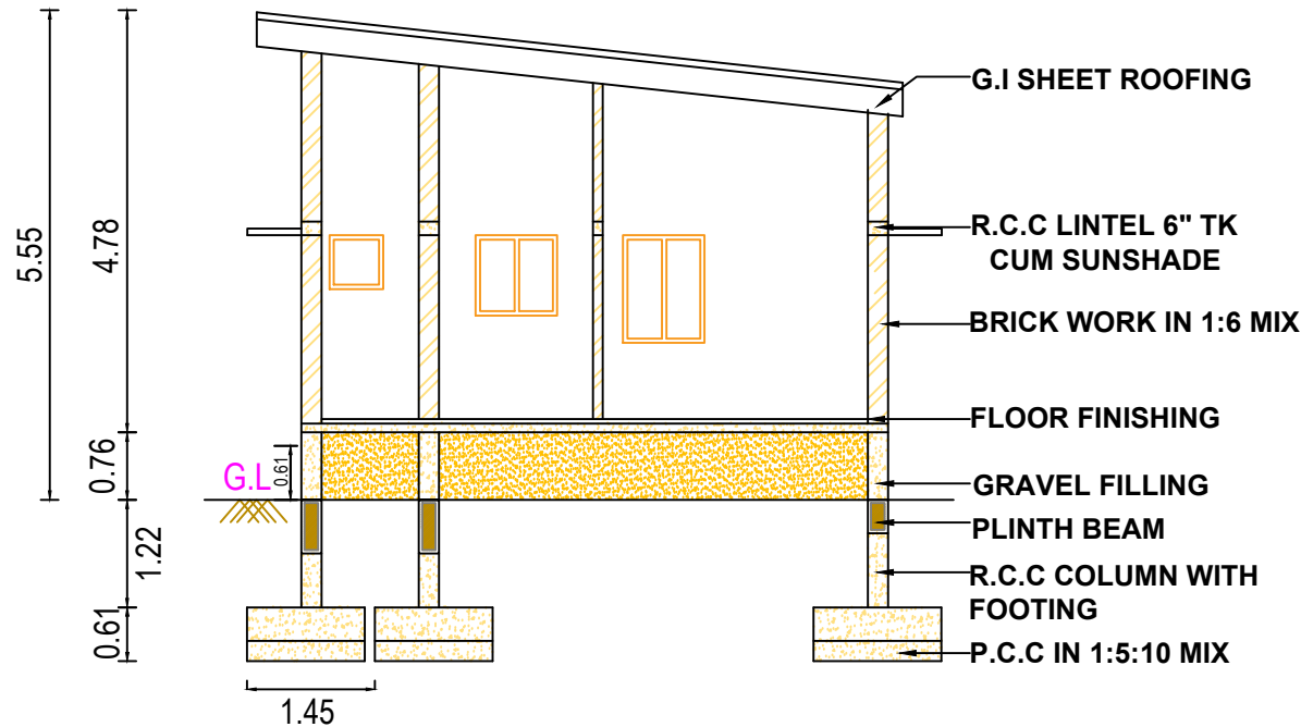
CROSS SECTION AT A-A
