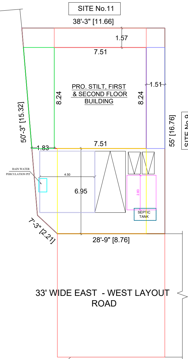
SITE PLAN
