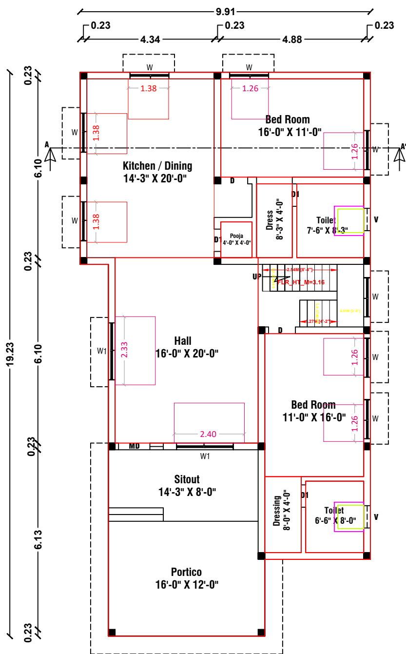
EXI.GROUND FLOOR PLAN
