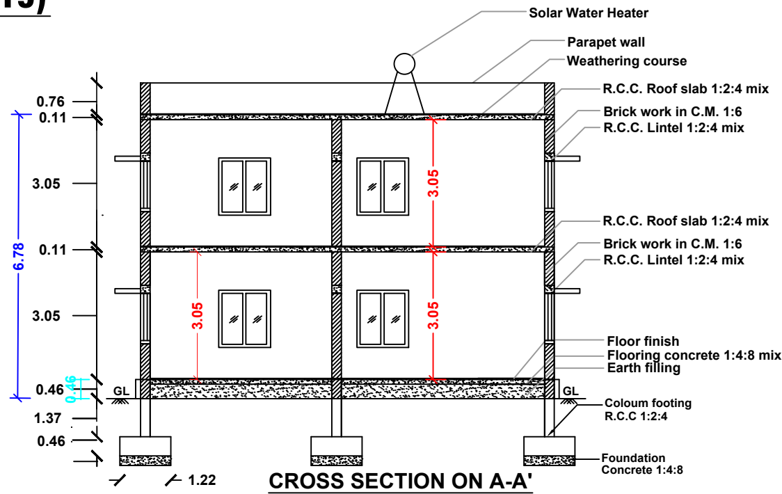
CROSS SECTION ON A-A'
