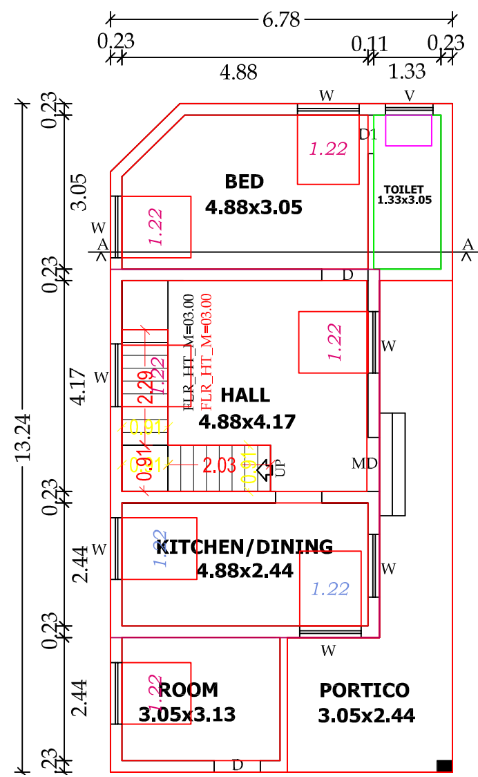
ND FLOOR PLAN
