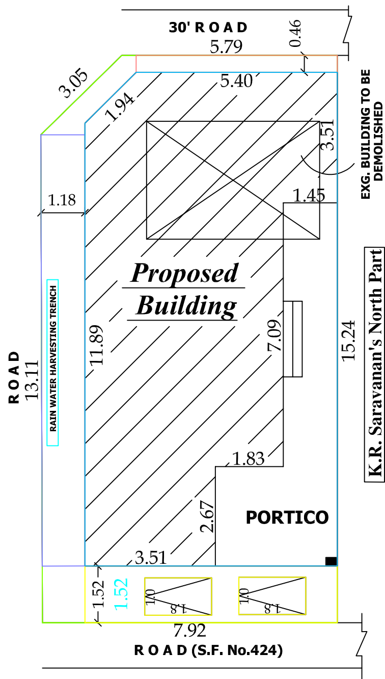
SITE PLAN
