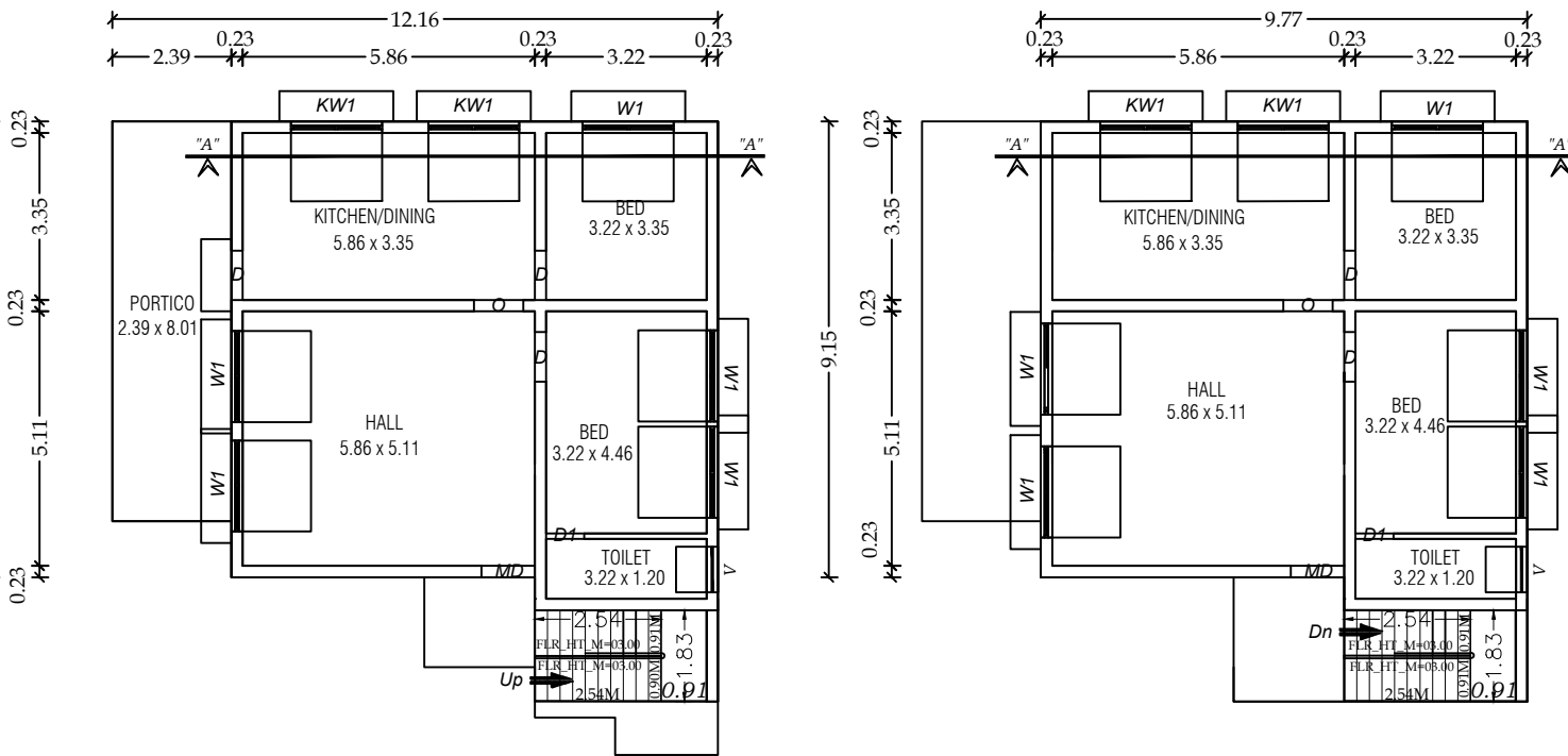
EX. GROUND FLOOR PLAN
