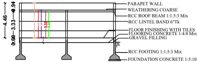
SECTION ON A-A SCALE 1:100
